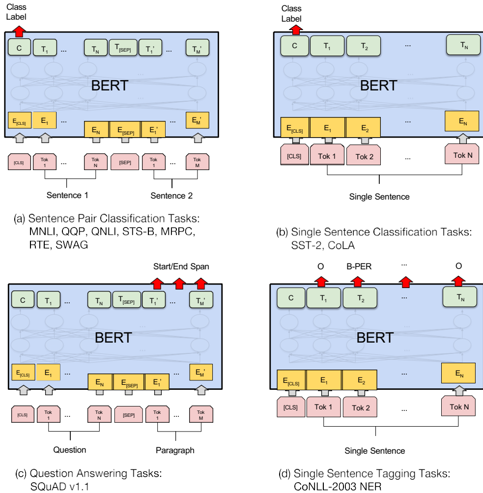
Figure 4: Illustrations of Fine-tuning BERT on Different Tasks.
